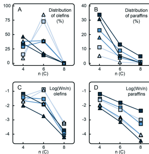
Fig. 10 The increase of Ti loading in the Phillips-type catalyst (from light to dark blue) shifts the selectivity towards C4 at the expense of C6 products in the experiments with ( \square ) and without ( \Delta ) hydrogen. A different trend in the distribution of olefinic species (A) compared to paraffinic species (B) is also clearly visible in the Schulz–Flory plots. While paraffinic species show linear curves independent of the Ti loading (D), olefin species exhibit a discrepancy from linearity with increasing Ti loading (C), indicating an oligomerisation mechanism, which does not follow SF distribution.
