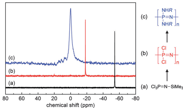
Fig. 4 Sample ^{31}\text{P}\{^1\text{H}\} NMR spectra of the monomer trichlorophosphoranimine \text{Cl}_3\text{P}=\text{N}-\text{SiMe}_3 (a), polydichlorophosphazene [\text{N}(\text{PCl}_2)_n] (b) and a macrosubstituted poly(organo)phosphazene [\text{N}(\text{NHR})_2]_n (c) demonstrating the simple tracking of the reaction progression. Adapted from H. Henke et al. , J. Polym. Sci., Part A: Polym. Chem. , 2013, 51 , 4467. Copyright 2013 Wiley Periodicals, Inc. 12
