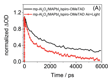
Fig. 5 Time-resolved transient absorption at 780 nm for pristine mp-Al 2 O 3 /MAPbI 3 /spiro-OMeTAD (black) and exposed to air and ambient light MAPbI 3 /spiro-OMeTAD (red) films. Traces normalized to \Delta OD = 1 at 1 ps time-delay to highlight differences in recombination kinetics. Laser excitation energy density = 25 \mu J cm -2 at 567 nm.
