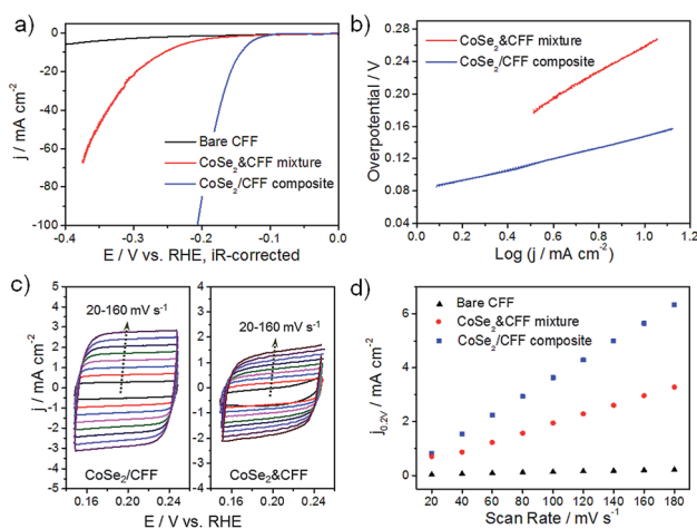
Fig. 3 Electrochemical performance of CoSe 2 /CFF electrode in 0.5 M H 2 SO 4 . (a) iR-corrected polarization curves for HER on bare CFF, CoSe 2 & CFF mixture and CoSe 2 /CFF composite, respectively; (b) Tafel plots and (c) cyclic voltammograms for CoSe 2 /CFF composite and CoSe 2 & CFF mixture at different scan rates from 20 to 160 mV s -1 , respectively; (d) the capacitive currents at 0.20 V vs. RHE as a function of scan rate for CoSe 2 & CFF mixture and CoSe 2 /CFF composite.
