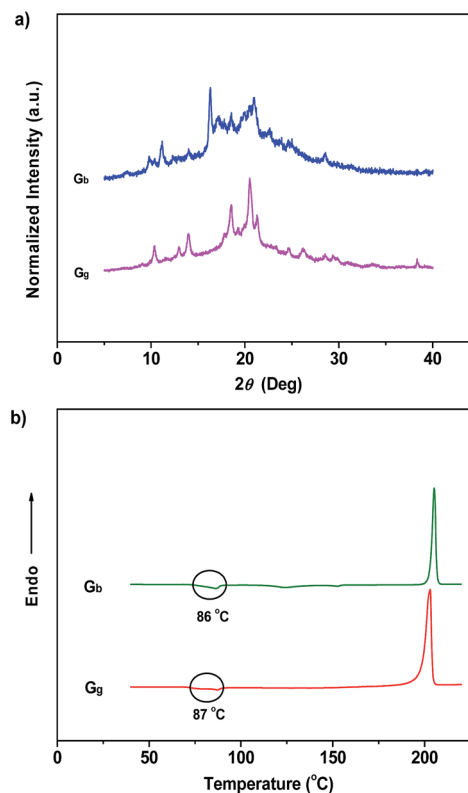
Fig. 6 XRD patterns (a) and DSC curves (b) of the ground samples of \text{P}_4\text{TA} : ( \text{G}_{\text{b}} ) ground sample from the blue-light crystals; ( \text{G}_{\text{g}} ) ground sample from the green-light crystals.
