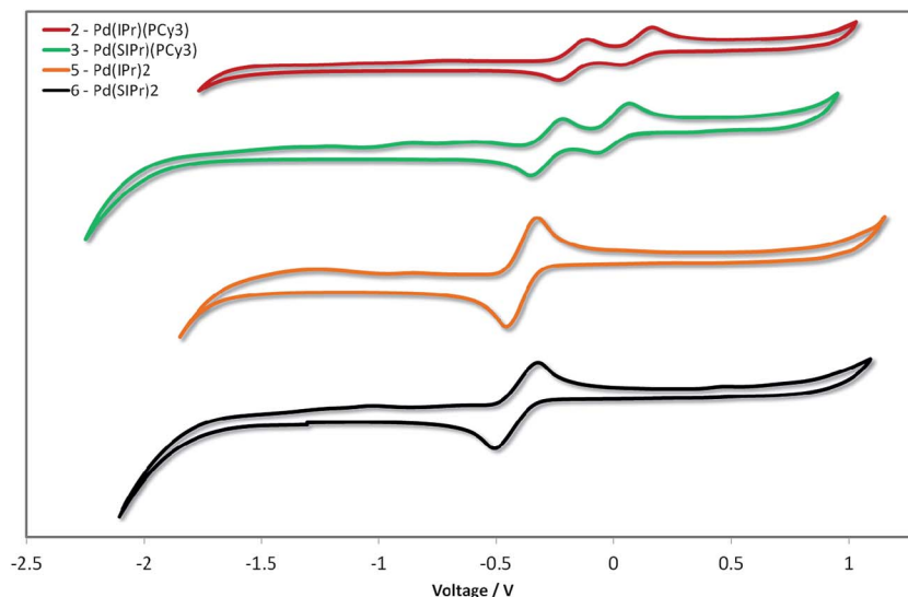
Fig. 10 Stacked cyclic voltammograms of 2 , 3 , 5 and 6 in degassed THF using a platinum disk working electrode, platinum wire counter-electrode, a \text{Ag}/\text{Ag}^+ pseudo-reference electrode and referenced vs. SCE using \text{Fc}/\text{Fc}^+ as an internal standard (0.56 V in THF). 46 Scan rate: 50 \text{ mV s}^{-1} .
