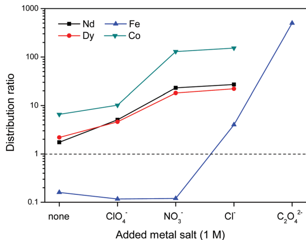
Fig. 11 Influence of added metal salts (1 M) with varying anions on the distribution ratio of Nd(III), Dy(III), Fe(III) and Co(II) ions in a biphasic [Hbet][Tf 2 N]-H 2 O system. A high distribution ratio corresponds to a greater affinity for the water phase. Oxalate forms highly insoluble complexes with REE(III) and Co(II) ions.
