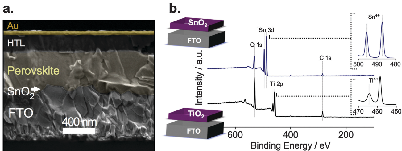
Fig. 2 Photovoltaic device architecture and elemental composition of the electron selective layers (ESLs). (a) Cross-sectional scanning electron micrograph of a typical layered photovoltaic device composed of FTO, \text{SnO}_2 as the electron selective layer (ESL), the perovskite film, a hole transporting layer (HTL, Spiro MeOTAD), and a gold top electrode. (b) X-ray photoelectron spectroscopy of \text{TiO}_2 and \text{SnO}_2 thin layers used as ESLs.
