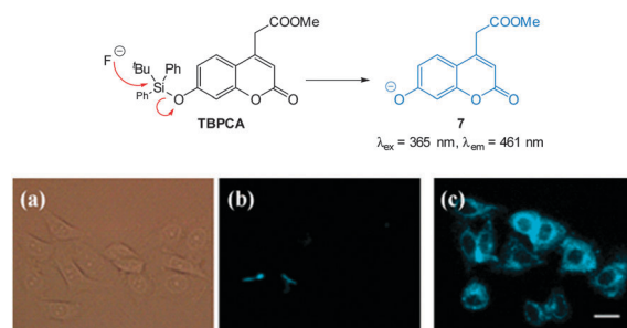
Fig. 7 Structure and reaction of coumarin TBPSCA with fluoride. (a) Bright-field image of A549 cells with TBPSCA (b) fluorescence image with TBPSCA without NaF (c) fluorescence image with TBPSCA and NaF. Scale = 20 \mu\text{m} . Reproduced with permission. 120
