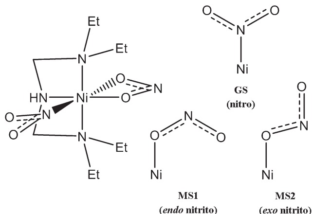
Fig. 1 Schematic structure of the [\text{Ni}(\text{Et}_4\text{dien})(\eta^2\text{-O,ON})(\eta^1\text{-NO}_2)] system. The four skeletal drawings show the structure of the molecule (left) and the three different binding modes of the isomerisable \text{NO}_2 group (right), viz. the ground-state (GS) nitro and metastable endo - and exo -nitrito forms (MS1/MS2, respectively).
