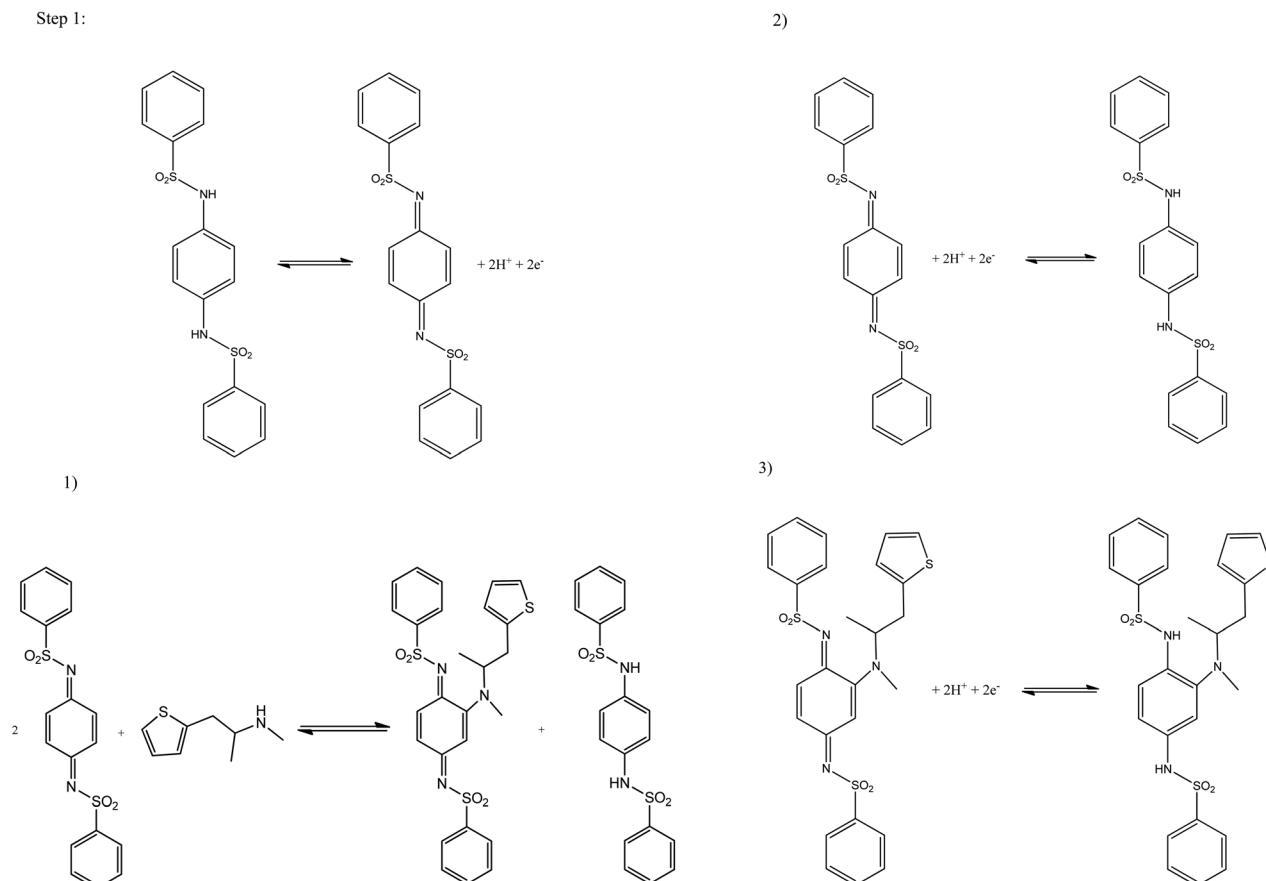
Scheme 1 Proposed indirect electrochemical methodology for the sensing of MPA. Step 1: Electrochemical process: Electrochemical oxidation of mediator appears at +0.07\text{ V} (vs. Ag/AgCl). (1) Chemical step: Reaction of MPA with the sulfonimide (oxidized form of the mediator). (2) Electrochemical step: Reduction of sulfonimide (oxidized form of the mediator) appears at -0.01\text{ V} (vs. Ag/AgCl). (3) Electrochemical step (analytical signal): reduction of the MPA with the sulfonimide intermediate appears at -0.36\text{ V} (vs. Ag/AgCl).
