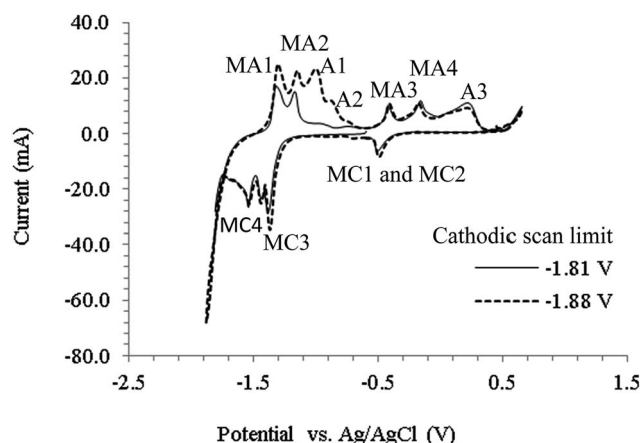
Fig. 3 Cyclic voltammograms obtained using a stainless steel wire working electrode in a molten \text{Li}_2\text{CO}_3\text{--Na}_2\text{CO}_3 electrolyte (molar ratio of 52 : 48) at 627 °C, at a scan rate of 100\text{ mV s}^{-1} , for negative potential limits of -1.81 V and -1.88 V. Atmosphere: \text{CO}_2 ; WE diameter: 0.25 mm; WE immersion depth: ca. 1.5 cm; CE: 6 mm diameter stainless steel rod; RE: alumina membrane \text{Ag/AgCl} .
