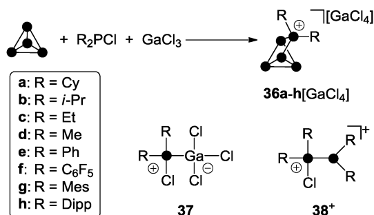
Scheme 10 Preparation of compounds 36a–h [GaCl 4 ] from P_4 , R_2PCL and GaCl_3 in fluorobenzene (R = aryl) or according to a solvent free approach (R = alkyl) and species 37 and 38 + commonly observed in mixtures of R_2PCL and GaCl_3 .
