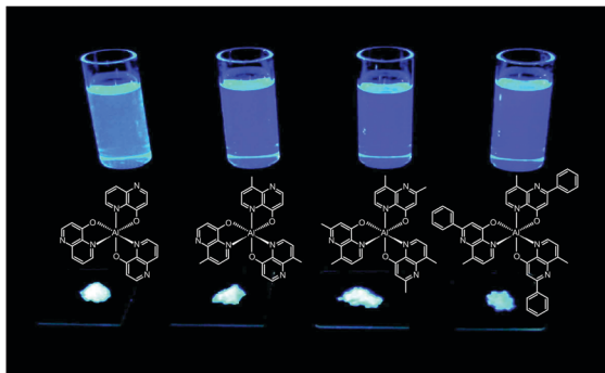
Fig. 5 Emission images of AlND 3 , AlmND 3 23 , AlmND 3 24 , and AlmpND 3 25 recorded in solution and solid state under irradiation by UV light. (Reproduced with permission from ref. 16. Copyright 2009, American Chemical Society.)
