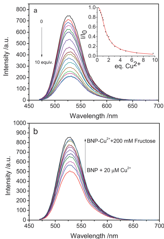
Fig. 2 (a) Fluorescence spectra of BNP ( 1 \times 10^{-5} M) in methanol in the presence of different concentrations of Cu 2+ (0–10 μM) with an excitation at 450 nm. Inset: fluorescence intensity at 525 nm of BNP as a function of Cu 2+ concentration. (b) Fluorescence spectra of BNP-Cu 2+ ( 1 \times 10^{-5} M) in the presence of different concentrations of fructose when excited at 450 nm.
