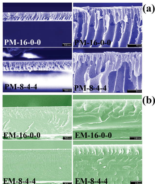
Fig. 3 Cross-section views for PES and modified PES membranes. (a) For the phase-inversion membrane, blue colour images, the scale bar is 50 \mu\text{m} (left) and 5 \mu\text{m} (right); (b) for the evaporation membrane, green colour images, the scale bar is 50 \mu\text{m} (left) and 10 \mu\text{m} (right).
