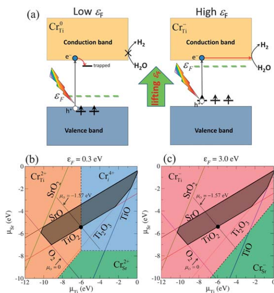
Fig. 1 (a) Schematic illustration of the effect of shifting \epsilon_F towards the conduction band on the stabilization of a low oxidation state of the Cr ion associated with \text{Cr}_{\text{Ti}} in Cr-doped STO. The energy levels of the in-gap Cr d states are shown. The arrows indicate the electron occupation corresponding to the associated charge state. (b) and (c) Illustrations of the conditions under which various Cr-related defects are stable, derived from the formation energy, with respect to the chemical potentials of Sr and Ti for (b) \epsilon_F = 0.3 eV ( p -type STO) and (c) \epsilon_F = 3.0 eV ( n -type STO). For the growth of STO under thermal equilibrium, \mu_{\text{Sr}} , \mu_{\text{Ti}} , and \mu_{\text{O}} must lie in the dark-shaded region.
