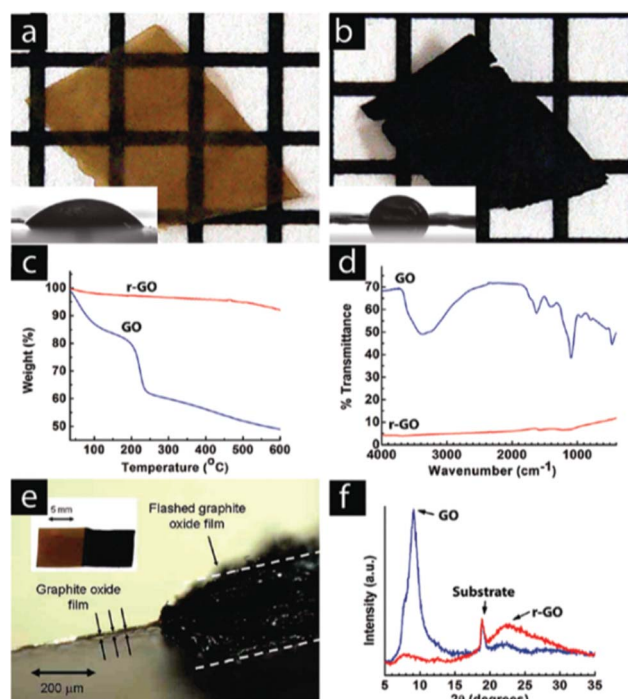
Fig. 16 A GO paper (a) can be instantaneously reduced (b) upon exposure to a photographic camera flash. The grids in the background are 1 \text{ mm} \times 1 \text{ mm} . The flash reduction of GO was evident by the dramatic changes in color (a, b), water contact angle (insets), (c) TGA, and (d) FTIR. In (c), (d) and (f) the blue lines correspond to GO and the red lines correspond with the flash-reduced GO. (e) Cross-sectional view of a RGO paper showing large thickness expansion after flash reduction. Only the right half of the GO sample was flashed. The left part of the picture shows the cross-sectional view of the light brown colored GO film. The thickness increased by almost 2 orders of magnitude, resulting in a very fluffy and potentially high surface area film. (f) The lack of a graphitic peak in the XRD pattern of the reduced material suggests disordered packing of the RGO sheets, consistent with the large volume expansion observed in (e). Reprinted with permission from ref. 176. Copyright (2009) American Chemical Society.
