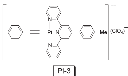
Fig. 13 The N^*N^*N Pt(II) acetylide complex Pt-3 used for TTA upconversion. The upconversion with Pt-3 was reported in ref. 35.
