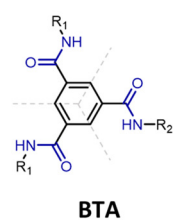
Fig. 1 Overview of benzene-based supramolecular motifs from earlier studies with identical hydrogen bonding units, highlighting structural features alongside a modified design for formation of BDUA with a C_2 -symmetric core motif. 35–37,39,40
