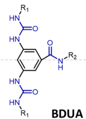
Fig. 1 Overview of benzene-based supramolecular motifs from earlier studies with identical hydrogen bonding units, highlighting structural features alongside a modified design for formation of BDUA with a C_2 -symmetric core motif. 35–37,39,40
