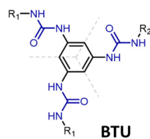
Fig. 1 Overview of benzene-based supramolecular motifs from earlier studies with identical hydrogen bonding units, highlighting structural features alongside a modified design for formation of BDUA with a C_2 -symmetric core motif. 35–37,39,40
