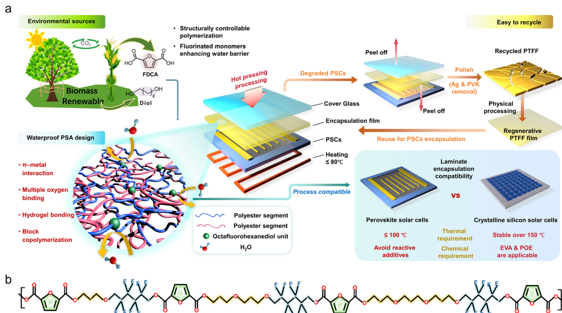
Fig. 1 Synthesis of PTFF and product screening. (a) Design principle of recoverable PTFF for PSCs nondestructive encapsulation. (b) Molecular structure of PTFF.
