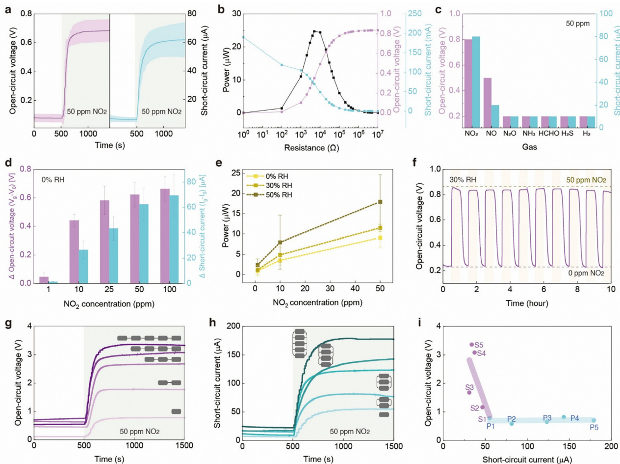
Fig. 3 Electrical performance of the GCEG. (a) Measured V_{OC} and I_{SC} profiles of the GCEG (20 k \Omega load) under 50 ppm NO 2 exposure at 0% RH. (b) Variation of V_{OC} , I_{SC} , and power output with external load resistances ranging from 1 \Omega to 10 M \Omega under 50 ppm NO 2 exposure at 50% RH. (c) Gas selectivity of the GCEG evaluated by comparing the maximum V_{OC} and I_{SC} under 50 ppm exposure to different gases at 0% RH. (d) Dependence of output voltage and current on NO 2 concentration (0–100 ppm) at 0% RH. (e) Variation of power output with NO 2 concentration and RH. (f) Long-term stability of the GCEG under cyclic adsorption–desorption of 50 ppm NO 2 at 30% RH. (g) Voltage and (h) current output from the five GCEG devices connected in series and parallel, respectively. (i) Enhanced output performance achieved by connecting multiple GCEG devices in series or parallel configurations under 50 ppm NO 2 exposure at 0% RH.
