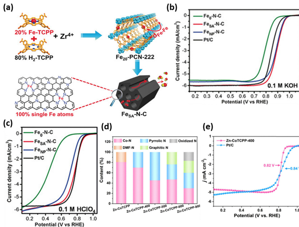
Fig. 5 (a) Schematic representation of the synthetic route for obtaining the Fe–N–C catalyst using MOF-545, including FeTCPP and H 2 TCPP moieties. Linear sweep voltammies obtained for the MOF-545-derived catalysts in (b) alkaline and (c) acidic media. Reproduced from ref. 100 with the permission from John Wiley and Sons, copyright 2018. (d) Normalized content of deconvoluted N-species quantified by high-resolution N 1s XPS. (e) LSV curves for the Zn–CoTCPP-400 electrocatalyst in O 2 -saturated 0.1 M KOH. Reproduced from ref. 101 with the permission from Elsevier, copyright 2025.
