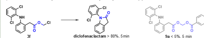
Fig. 4 (A) Expanding the scope of precursors: utilization of chloromethyl esters of pivalic acid ( 3b ), N -boc-baclofen ( 3c ), ibuprofen ( 3d ) and cinnamic acid ( 3e ) for the synthesis of various acylals shows similar outcome as in the first series. (B) Failed approach in synthesis of diclofenac acylals from chloromethylester of diclofenac ( 3f ): thermodynamically favoured reactions, such as lactam formation, limit the reaction protocol, but proceed independently of the solvent used.
