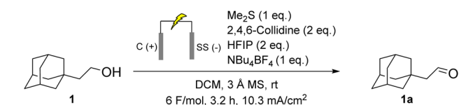
Scheme 2 Standard reaction conditions for the eCarbonyls reaction.
