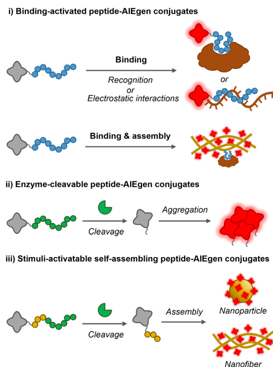
Fig. 1 Schematic illustration of design strategies for activatable peptide-AIEgen conjugates for cancer imaging.
