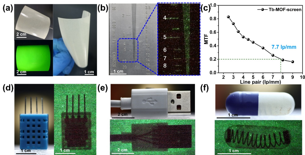
Fig. 4 (a) The photographs of the flexible Tb-MOF-screen. (b) Profile displays (left) and X-ray images (right) of the standard line pair card. (c) MTF of the X-ray image based on the standard line pair card. The real pictures and X-ray radiographs of the electronic component (d), the USB connector (e), and the capsule (f).
