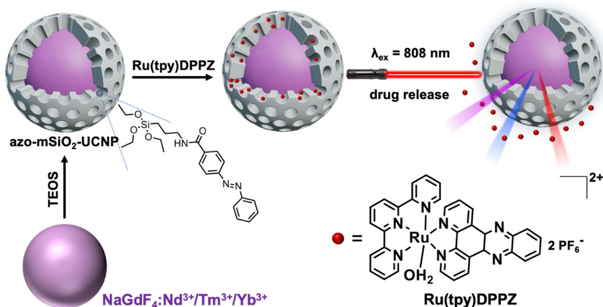
Fig. 1 Preparation of Ru(tpy)DPPZ loaded azo-mSiO 2 -UCNP nanohybrids and NIR-photoactivated drug release. TEOS = tetraethyl orthosilicate; tpy = 2,2':6',2''-terpyridine; DPPZ = dipyrrolo[3,2- a :2',3'- c ] phenazine.
