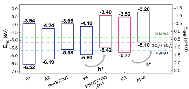
Fig. 11 Energy level alignment of conjugated polymers and small molecules for photoanode with redox potential of dehydroascorbic acid (DHA)/ascorbic acid (AA), SO 3 2- /SO 3 - (sacrificial agents) and H 2 O/O 2 .
