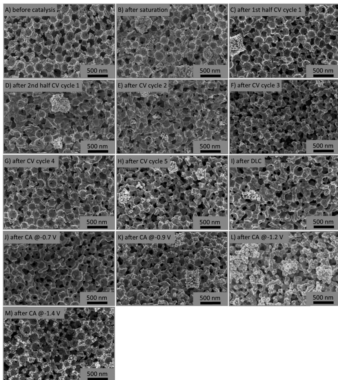
Fig. 10 HR-SEM Images of the porous p-flat-default electrode (A) before catalysis; (B) after saturation (10 mL CO 2 per min for 1 h); (C) after the first half CV cycle (0.1 → -1.4 vs. RHE); (D) after the second half CV cycle ( -1.4 → 0.1 vs. RHE); (E) after the second CV cycle; (F) after the third CV cycle; (G) after the fourth CV cycle; (H) after the fifth CV cycle; (I) after DLC; (J) after catalysis at -0.7 V vs. RHE; (K) after catalysis at -0.9 V vs. RHE; (L) after catalysis at -1.2 V vs. RHE and (M) after catalysis at -1.4 V vs. RHE.
