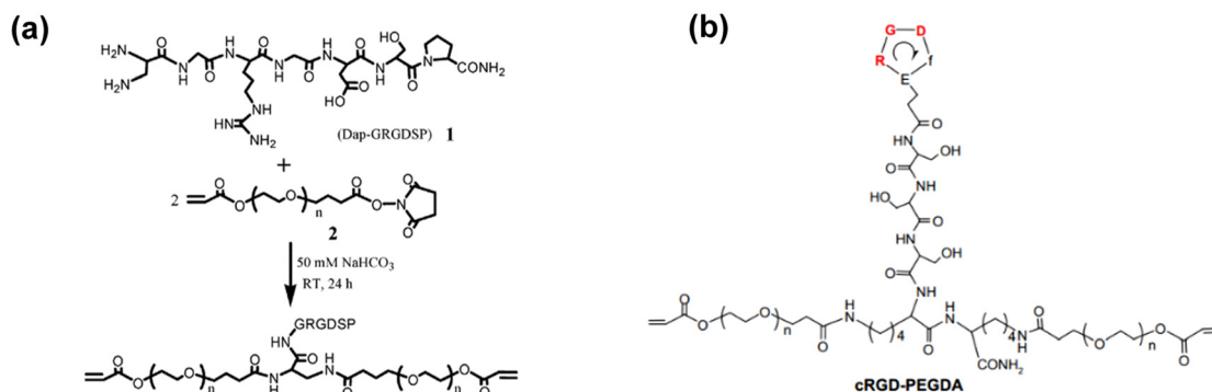
Fig. 3 Synthesis of RGD-incorporated PEGDA (RGD-PEGDA) (a) by conjugation of diaminopropionic acid (Dap)-capped GRGDSP and Acryl-PEG-NHS (reproduced from ref. 51 with permission from American Chemical Society, copyright 2006). (b) Constructed by a hydrophilic tail with a spacer of three serine residues (SSS) and a linker of two lysine residues (KK), and cRGD-incorporated PEGDA (cRGD-PEGDA) (reproduced from ref. 35 with permission from Elsevier, copyright 2010).
