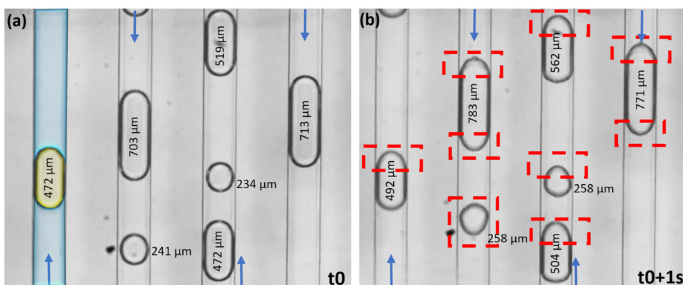
Fig. 14 A close-up view of the CO 2 gas bubbles at 15 bar before ( t_0 ) and after hydrate formation ( t_0 + 1 s). (a) CO 2 bubbles in water with the flow direction indicated by blue arrows. One line is colored for better visualization of conditions: green represents the CO 2 bubbles, blue represents the water; (b) hydrate crystallization, highlighted with red boxes.
