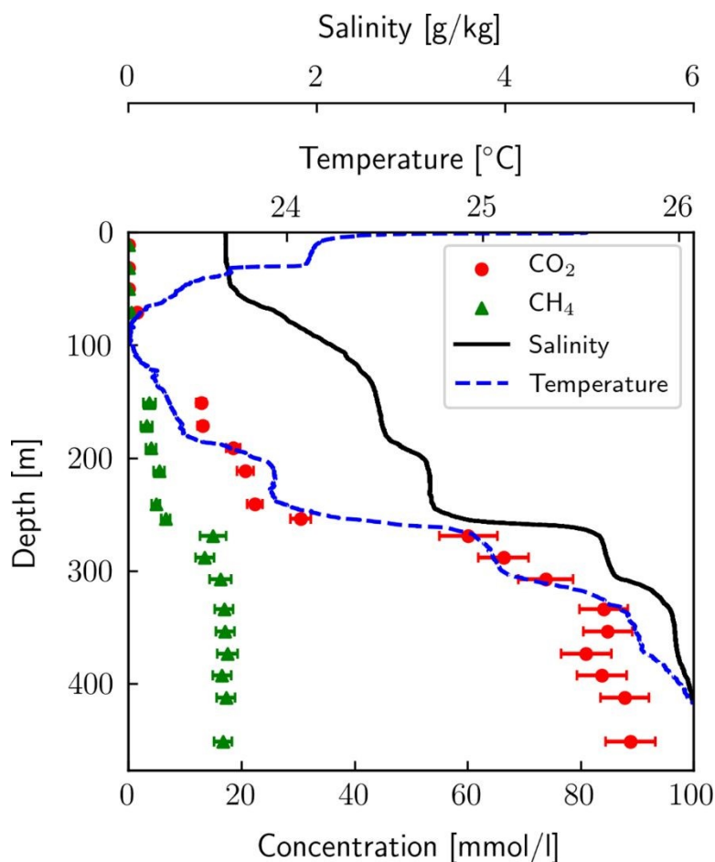
Fig. 2: Vertical profiles of temperature, salinity, and dissolved \text{CH}_4 and \text{CO}_2 concentrations in Lake Kivu. Reprinted (adapted) from reference 24. Copyright 2020 The Authors. 24
