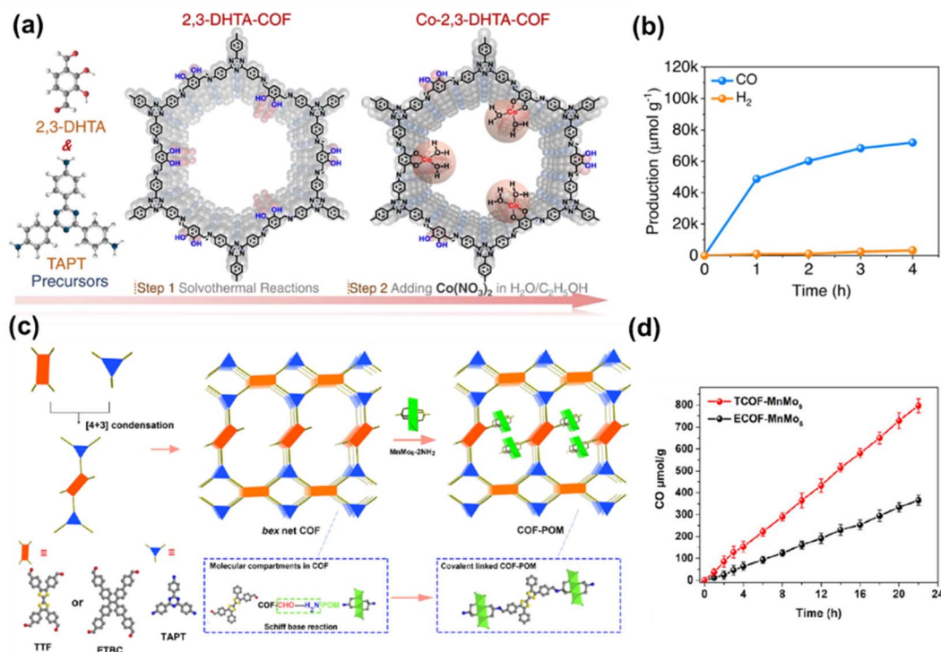
Fig. 11 (a) Synthesis of 2,3-DHTA-COF and Co-2,3-DHTA-COF. (b) CO and \text{H}_2 evolution with irradiation time for the \text{CO}_2\text{RR} catalyzed by Co-2,3-DHTA-COF under visible light irradiation. Adapted with permission. 111 Copyright 2023, Springer Nature. (c) Schematic of uniformly dispersed POM clusters in the COF by confining them into the pores of the COF through covalent linkages. (d) Time-dependent \text{CO}_2 -to-CO performance for TCOF-MnMo 6 and ECOF-MnMo 6 . Reproduced with permission. 119 Copyright 2022, American Chemical Society.
