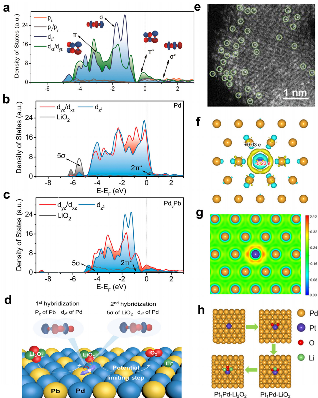
Fig. 13 (a) DOS of Pd d_{z^2} , d_{xz/yz} orbitals and Pb p_x , p_y , p_z orbitals after intra-molecular p-d orbital hybridization in \text{Pd}_3\text{Pb} . (b) DOS of Pd 4d d_{yz}/d_{xz} and d_{z^2} orbitals in Pd. (c) DOS of Pd 4d d_{yz}/d_{xz} and d_{z^2} orbitals in \text{Pd}_3\text{Pb} with adsorbed \text{LiO}_2 . (d) Schematic representation of cascade orbital-oriented hybridization from intra-molecular Pb-Pd p-d hybridization in \text{Pd}_3\text{Pb} to inter-molecular orbital hybridization between \text{Pd}_3\text{Pb} (Pd 4d_{xz/yz} and 4d_{z^2} ) and \text{LiO}_2 ( 2\pi^* and 5\sigma ), using the d_{z^2} orbital along the z-axis as an example. 115 (e) AC-HAADF-STEM image of the \text{Pt}_1\text{Pd} alloy (single-atom Pt marked with green circles). (f) ELF values of \text{Pt}_1\text{Pd} . (g) Charge density difference distribution (regions of electron enrichment and depletion) in \text{Pt}_1\text{Pd} . (h) Schematic representation of the discharge pathway of a Li-O 2 battery on the \text{Pt}_1\text{Pd} surface. 40
