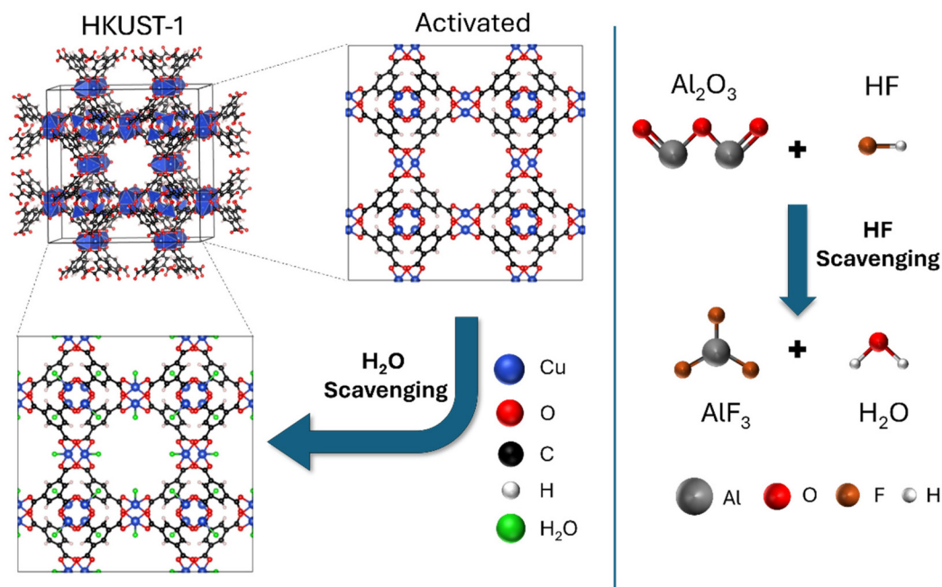
Fig. 2 Scavenging mechanism for \text{H}_2\text{O} and \text{HF} by HKUST-1 and \text{Al}_2\text{O}_3 nanoparticles, respectively.
