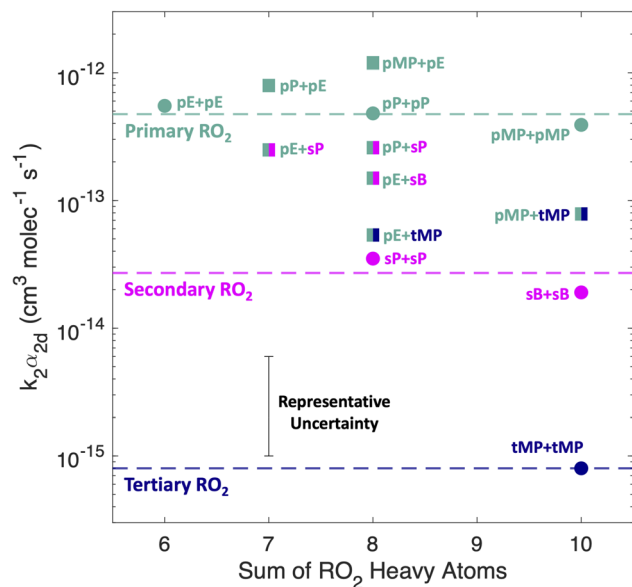
Fig. 4 Measured values of k_{2\alpha_{2d}} for the self-reactions of the ethene, methylpropene, propene, and cis -2-butene-derived peroxy radical systems, plotted as a function of the sum of the number of heavy atoms in the participating peroxy radicals and colored by substitution of the peroxy radical. Dashed lines give the average value of k_{2\alpha_{2d}} for each of the primary, secondary, and tertiary peroxy radical groups. Squares give k_{2\alpha_{2d}} values for the cross-reactions measured in this work. All points are labeled with the participating peroxy radicals.
