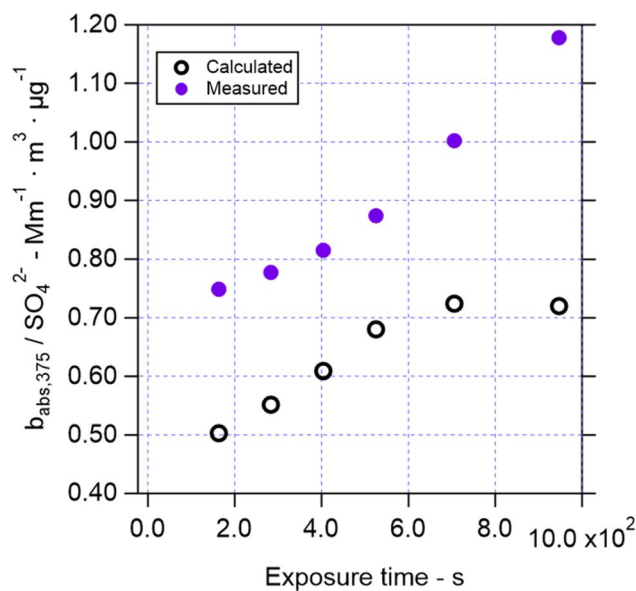
Fig. 4 Example of absorption coefficients (units of \text{Mm}^{-1} ) at 375 nm, with normalization by sulfate AMS loading (units of \mu\text{g m}^{-3} ) at \text{RH} = 25\% \pm 5\% , for the data in Fig. 2 and 3. The measured values were obtained from the aethalometer. The predicted values arise from the measurements of mass loading of NVA in the flow tube and the measured MAC value for NVA.
