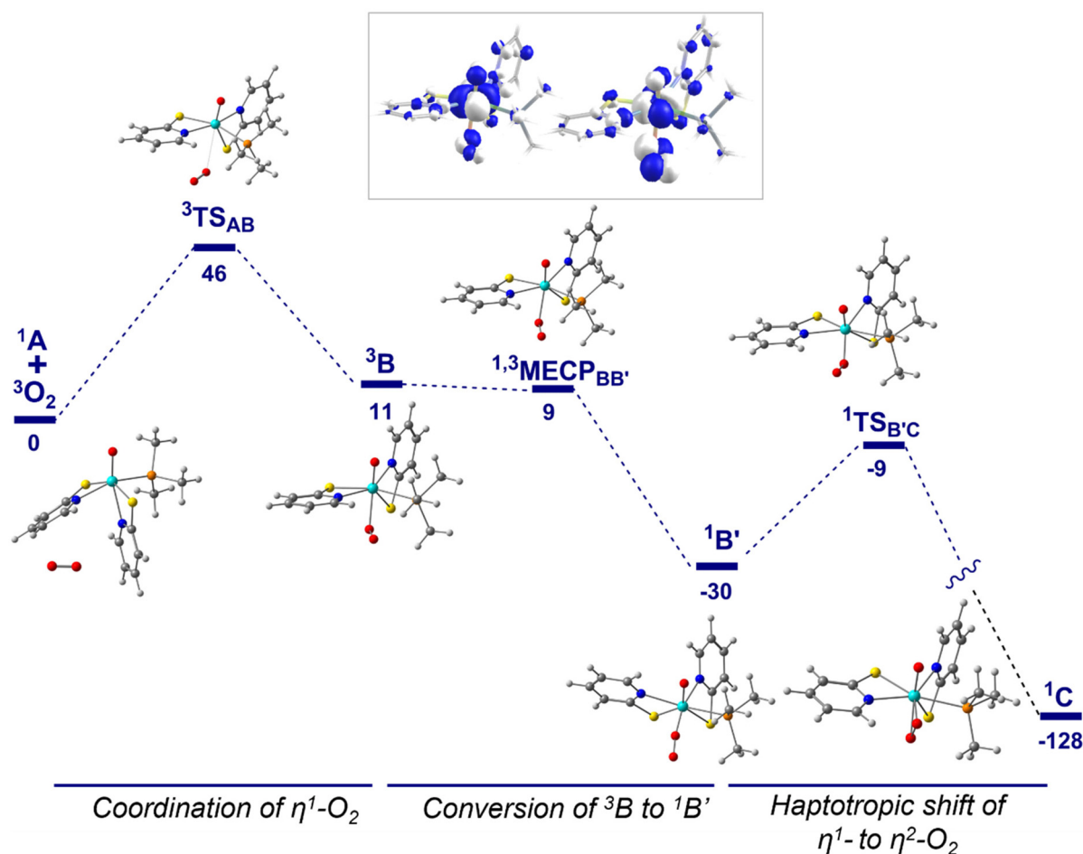
Fig. 2 Dioxygen activation: the interaction of {}^3\text{O}_2 with {}^1[\text{W}(\text{IV})\text{O}(\text{PyS})_2(\text{PMe}_3)] (A) and the quasi-restricted single occupied orbitals (SOMOs in the inset) of the complex at the triplet state of {}^{1,3}\text{MECP}_{\text{BB}'} (energies in \text{kJ mol}^{-1} ).
