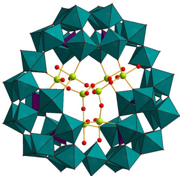
Fig. 11 Combined polyhedral/ball-and-stick representation of [\text{Rb}_3\text{C}\{\text{V}^{\text{IV}}\text{V}^{\text{V}}\text{O}_7(\text{H}_2\text{O})_6\}_2\{\text{H}_6\text{P}_6\text{W}_{39}\text{O}_{147}(\text{H}_2\text{O})_3\}]^{15-} . Color code: \text{WO}_6 octahedra (green), \text{PO}_4 tetrahedra (pink), O (red), V (yellow). 93
