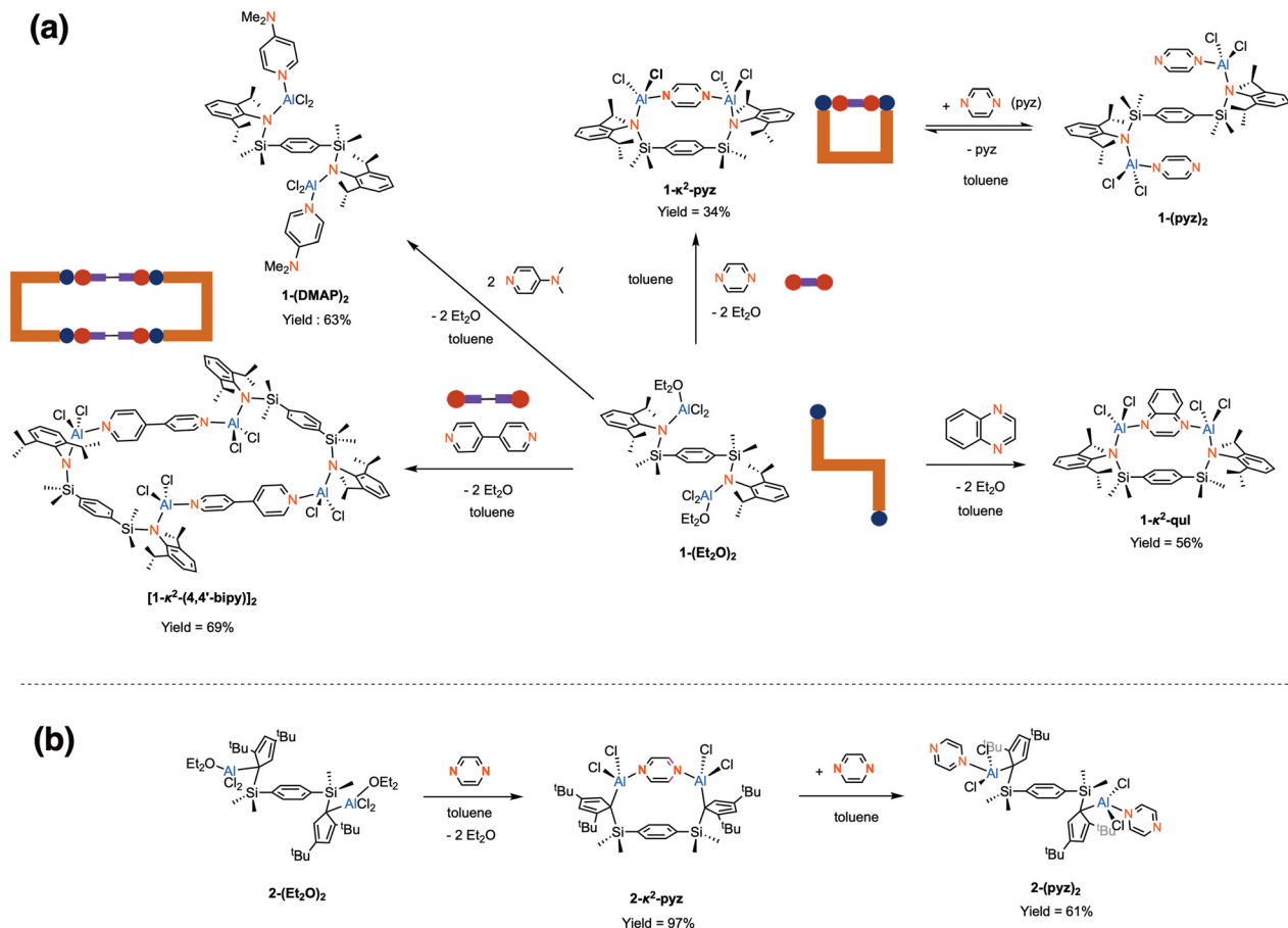
Scheme 2 Reactivity of (a) 1-(Et 2 O) 2 and (b) 2-(Et 2 O) 2 .
