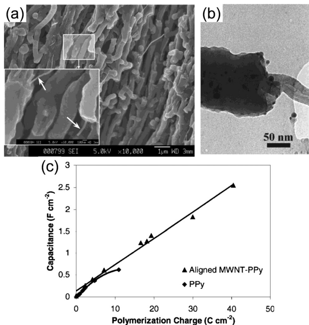
Fig. 6 (a) SEM images of vertically aligned CNTs coated with PPy via direct electro-deposition (deposition charge: 40\ C\ cm^{-2} ). The inset is an enlarged view showing the uncoated portions of the CNTs. (b) A single CNT with the left portion being coated with PPy and the right portion being naked. (c) Areal capacitance of PPy coated vertically aligned CNTs (triangles) and that of pure PPy (diamonds) as a function of deposition charge. Reproduced from ref. 92 with permission from John Wiley and Sons, copyright 2002.
