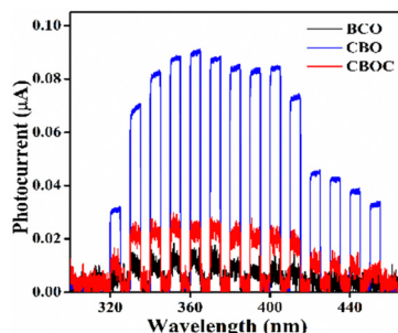
Fig. 4 Photocurrent generation at different wavelengths by applying 1 V and using 5 s open/close shutter.
