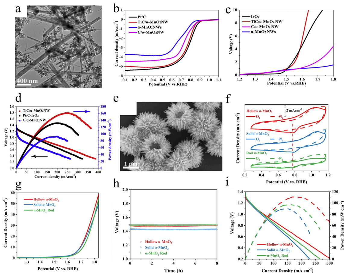
Fig. 8 The surface morphology and electrocatalytic performance. (a) The SEM image of TiC/α-MnO 2 NW prepared by a hydrothermal method. (b) LSV curves for the ORR, (c) LSV curves for the OER, and (d) discharge polarization curves of various catalysts. Reproduced with permission. 74 Copyright 2020, Elsevier. (e) The SEM image of the urchin-like α-MnO 2 prepared by a hydrothermal method. (f) CV polarization curves. (g) OER polarization curves. (h) Open-circuit plots, and (i) the discharge polarization curves and power density plots of the assembled zinc-air battery. Reproduced with permission. 75 Copyright 2022, Elsevier.
