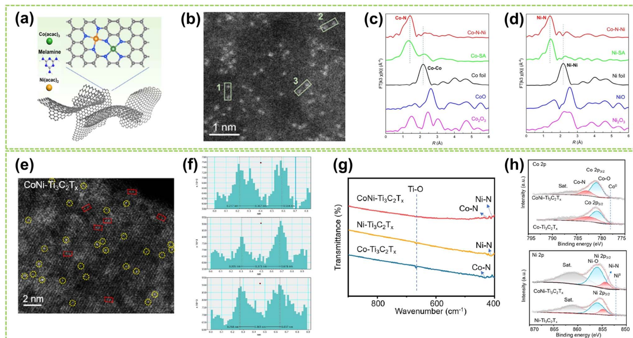
Fig. 5 Structure characterization of heteronuclear DACs connected by heteroatomic bridges. (a) Schematic diagram of the polymerization-pyrolysis synthesis method of Co-N-Ni. (b) AC HAADF-STEM image of Co-N-Ni. The bright spots in the green box represent the Co, Ni dual-atom. (c) Co K-edge and (d) Ni K-edge FT-EXAFS spectra of Co-N-Ni DAC, Co/Ni-SA, and the references 52 (reproduced with permission from ref. 52 copyright 2023, ACS). (e) HAADF-STEM images of CoNi-Ti 3 C 2 T x , where bright spots corresponding to single metal atoms are marked by yellow circles, and possible Co-Ni atomic pairs are highlighted by red rectangles. (f) Intensity profiles were obtained on adjacent metal atomic pairs, taken from three different sites marked by red rectangles in (e). (g) FTIR spectra of CoNi-Ti 3 C 2 T x , Ni-Ti 3 C 2 T x , and Co-Ti 3 C 2 T x composites. (h) Above: Co 2p and below: Ni 2p high-resolution XPS spectra of CoNi-Ti 3 C 2 T x and Co-Ti 3 C 2 T x composites 53 (reproduced with permission from ref. 53 copyright 2024, ACS).
