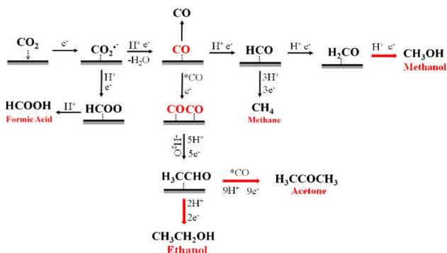
Fig. 8 Possible reaction pathways for the electrocatalytic CO 2 RR on the Cu/Co electrode.
