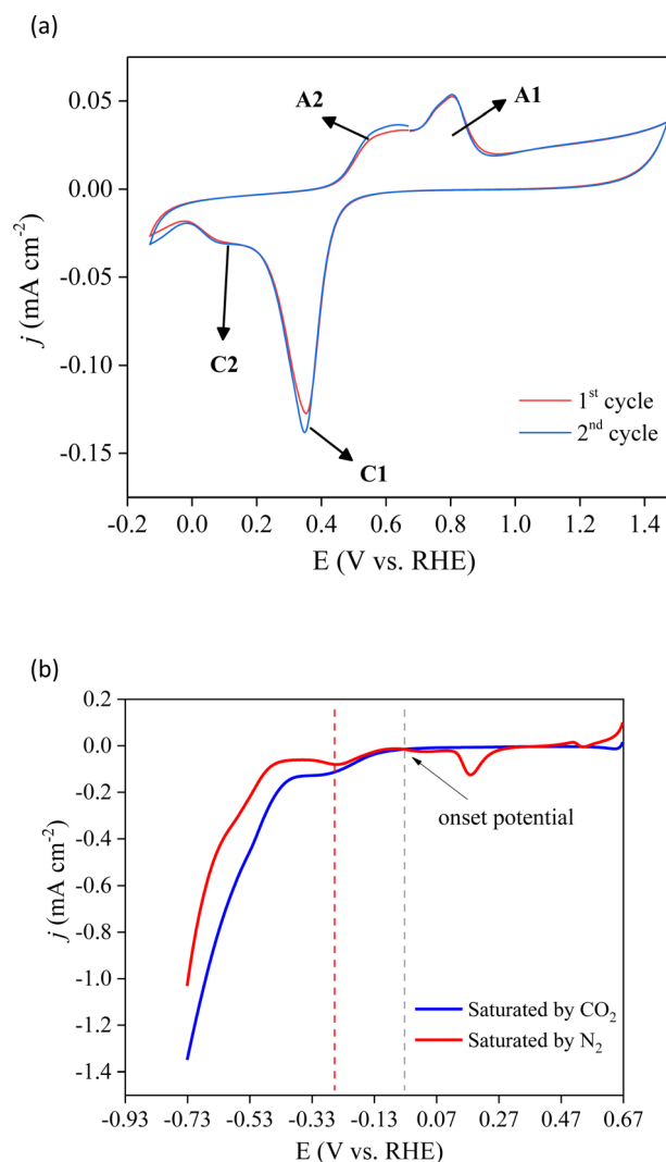
Fig. 5 Cyclic (a) and linear (b) voltammetry of the prepared Cu/Co electrode in 0.1 M Na 2 SO 4 under CO 2 and N 2 atmospheres at 25 \text{ mV s}^{-1} .
