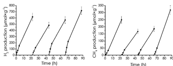
Fig. 5 Temporal hydrogen and methane evolution in the photocatalytic irradiation of CD-1/mpC in four consecutive uses. Reaction conditions: acetonitrile 12 mL, \text{H}_2\text{O} 4 mL, triethanol amine 4 mL, CD-1/mpC at 0.5 mg \text{mL}^{-1} , irradiation through quartz with the full output of a 300 W Xe lamp.
