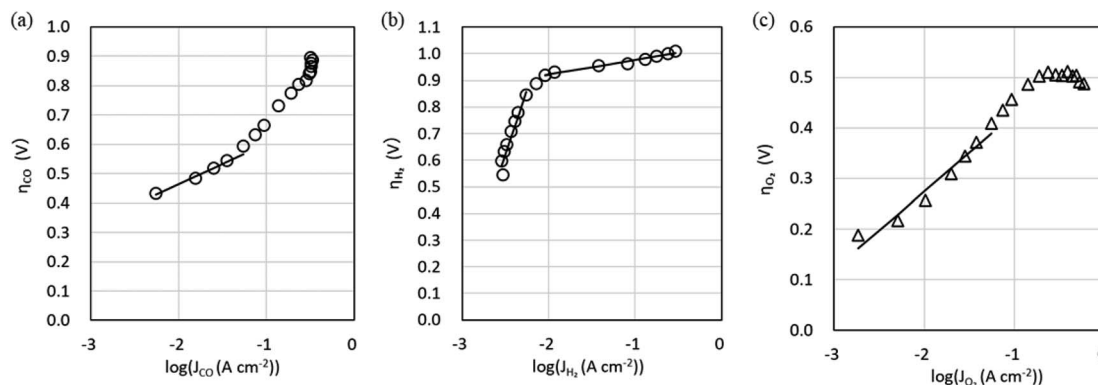
Fig. 5 Tafel plots at a \text{CO}_2 flow rate of 5 sccm \text{cm}^{-2} and cell temperature of 50 °C. (a) CO evolution reaction (COER). (b) \text{H}_2 evolution reaction (HER). (c) \text{O}_2 evolution reaction (OER).
