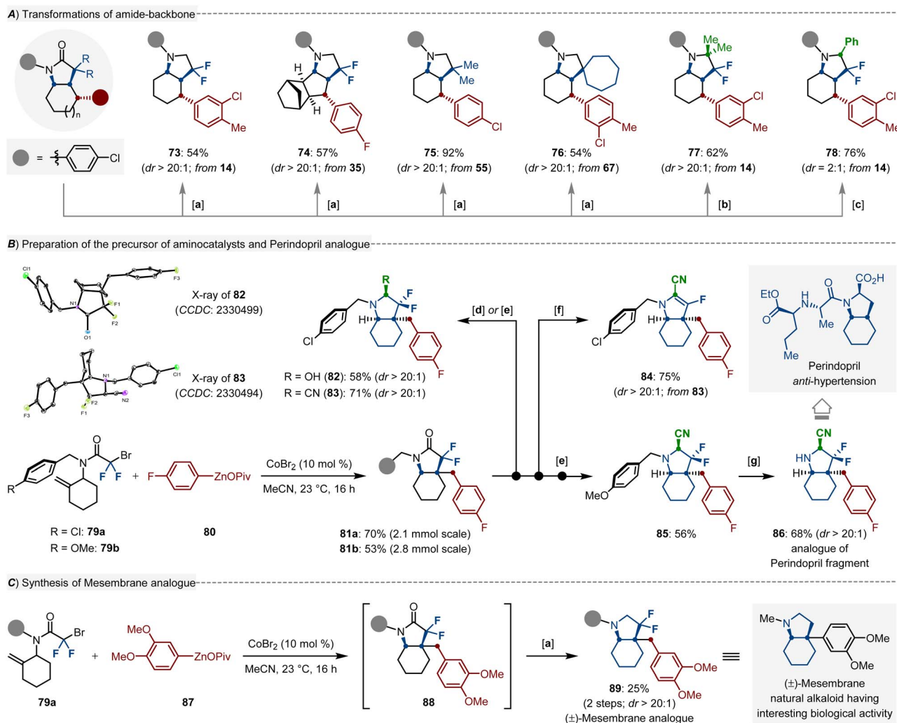
Scheme 4 Synthetic applications. (A) Functionalization of amide-backbones, (B) late-stage synthesis of medicinally relevant molecules, (C) preparation of analogue of mesembrine. Reaction conditions: [a] \text{Mn}(\text{CO})_5\text{Br} (2.0 mol%), \text{Ph}_2\text{SiH}_2 (2.0 equiv), THF, 80 °C, 4 h. [b] \text{MeLi} (1.0 equiv), \text{TiCl}_4 (1.0 equiv), and \text{MeLi} (2.0 equiv), Toluene. [c] (i) \text{NaH} (3.0 equiv), \text{NaI} (1.0 equiv), THF, 40 °C, 3 h; (ii) \text{TMSCl} (2.5 equiv), \text{PhMgCl} (2.0 equiv), 0 to 23 °C, 2 h. [d] (i) \text{NaH} (3.0 equiv), \text{NaI} (1.0 equiv), THF, 70 °C, 16 h; (ii) \text{TMSCl} (4.0 equiv), \text{Bu}_4\text{NCN} (2.0 equiv), 23 °C, 5 h. [e] (i) \text{DIBAL} (1.3 equiv), THF, −35 °C, 2 h; (ii) \text{TMSCN} (5.0 equiv), −35 to 20 °C, 1 h. [f] (i) \text{KOH} (2.0 equiv) in \text{H}_2\text{O} , 1,4-Dioxane, 115 °C, 3 h; (ii) then \text{HCl} . [g] TFA, anisole, 55 °C, 2 h.
