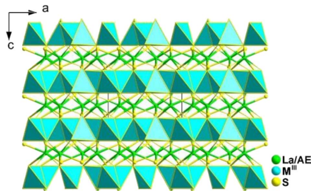
Fig. 9 Structure of \text{LaAE}^{\text{III}}\text{S}_7 along the b axis with the unit cell outlined.
